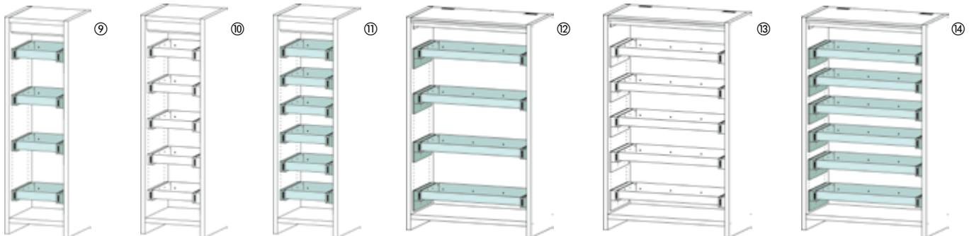
Type 6/20 with 4 full drawers (at 11 litres)
