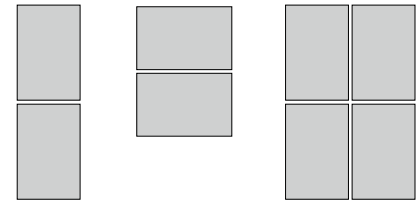
Covering strips and cover plate for multiple installation
