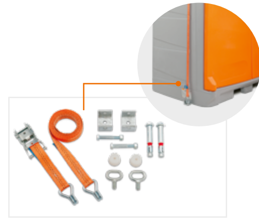
Wind load protection
