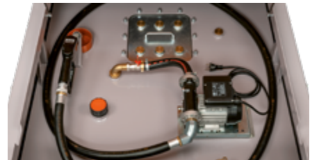
DT-Mobil PRO ST 980 Basic, with pump Cematic 72
