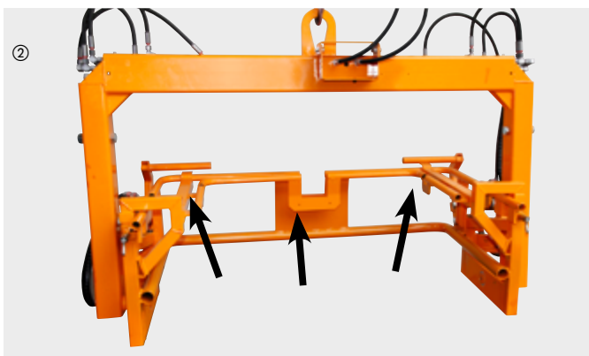
② Loading frame hydraulic, tilting with auxiliary frame, for grit bin 200 L
